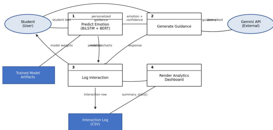
Data Flow Diagram — AI Learning Assistant
